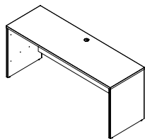
72W x 24D Desk/Credenza/Return OFD272XX $520.00
