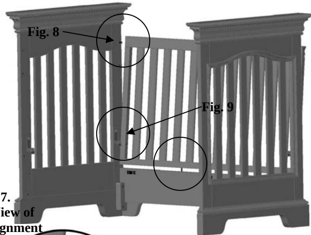
Figure 7. Align Crib Side
