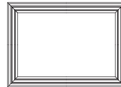
- 30 RECTANGULAR MIRROR Beveled plate: 42 1/8W 28 5/8H (107 x 73 cm) Overall: 48W 34 1/2H (122 x 88 cm)
